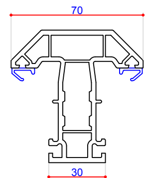
702503 (P10503) 70mm T Transom Steel Box 713187 (S00187)
