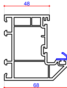
701532 (P10532) Chamfered Comp Door Outer Frame Aluminium Box 715406 (A00406)
