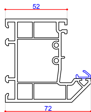
701502 (P10502) 72mm Outer Frame Steel Box 713191 (S00191) Steel P Section 713157 (S00157)
