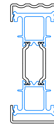
704811 (A70425) Thermally Broken Ali Coupler Sculptured Cover 716324 (P10324) Plain Cover 716323 (P10323)
