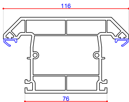
702505 (P10505) 116mm Midrail Steel U Channel 713166 (S00166)
